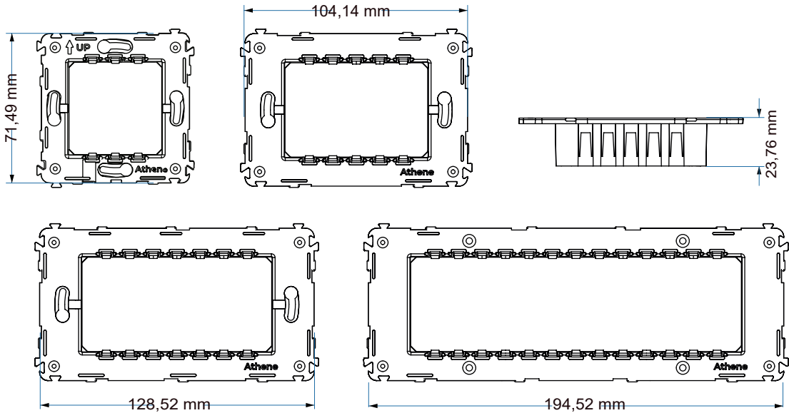
Mounting Plate *
